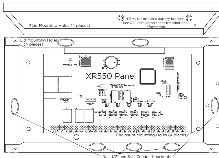
Figure 2: XR550 Series in Model 341 Enclosure
