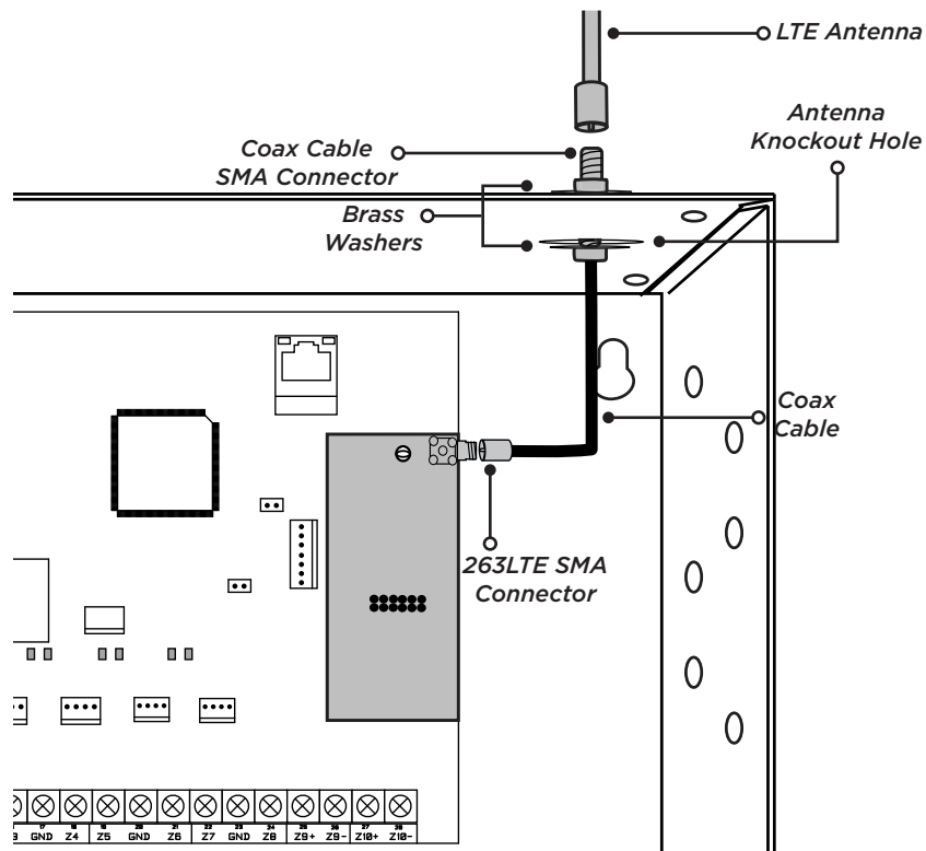
Figure 10: 263LTE Cellular Communicator Connection
