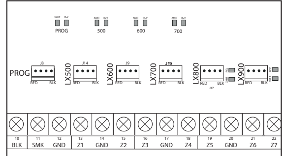
Figure 6: LX-Bus Headers and LEDs
