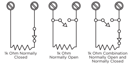
Figure 5: End-of-Line Resistors
