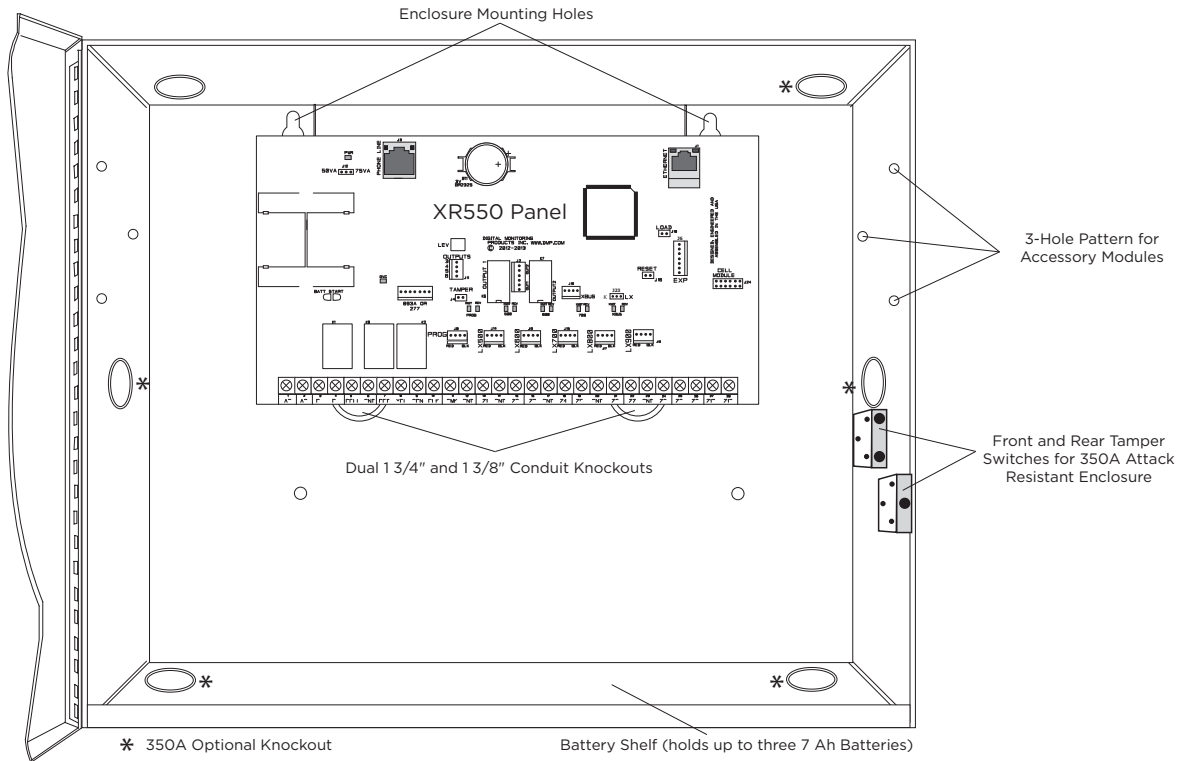
Figure 1: XR550 Series in Model 350 or 350A Enclosure
