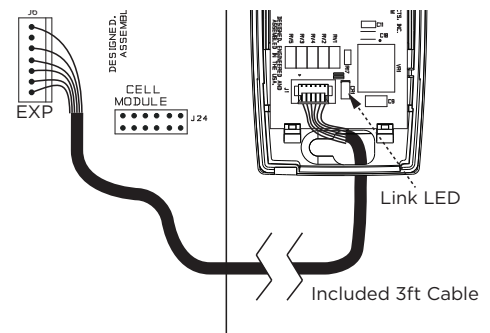
Figure 11: 763 to XR150/XR550 Series
