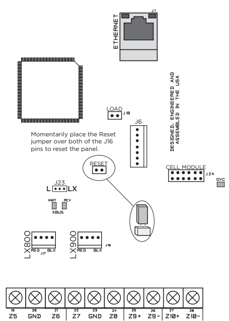
Figure 9: XR550 Series Panel Showing the RESET Jumper
