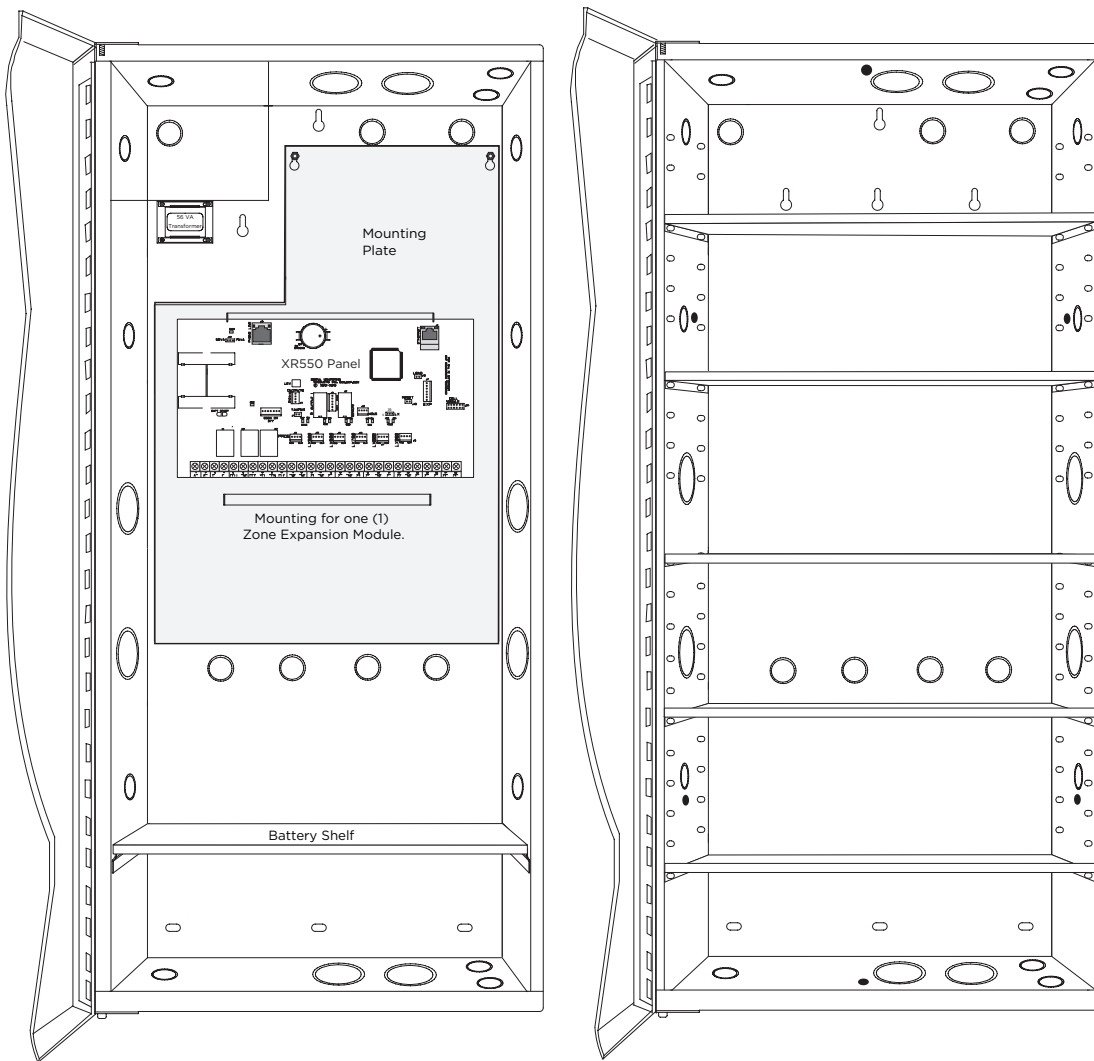
Figure 3: XR550 Series in Model 352X Enclosure and Separate 352S Enclosure with Shelves
