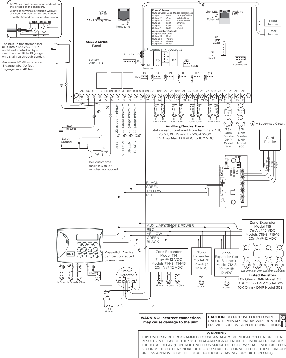
Figure 4: XR550 Series Wiring Diagram
