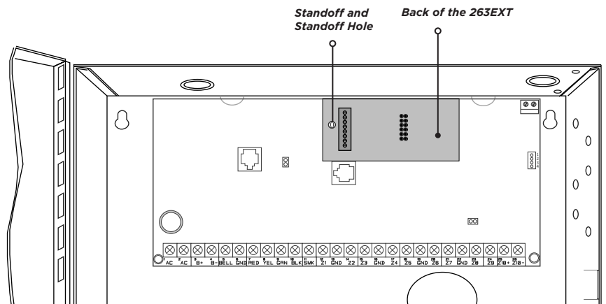
Figure 3: 263EXT Panel Module on an XT Series Control Panel
