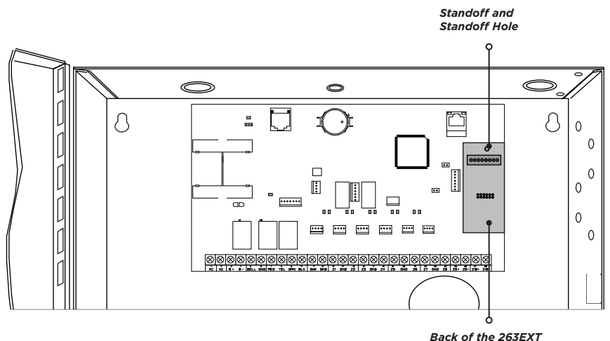
Figure 4: 263EXT Panel Module on an XR Series Control Panel
